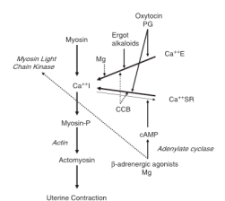
Fig. 1. A schematic overview of uterine contraction. Calcium, Ca 2+ ; I, intracellular; E, extracellular; SR, sarcoplasmic reticulum; Mg, magnesium; CCB, calcium channel blockers; PG, prostaglandins; cAMP, cyclic adenosine monophosphate. The dotted lines represent an inhibitory effect. Enzymes are printed in italic.
