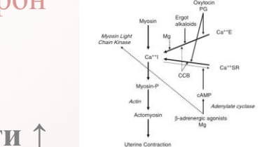
Fig. 1. A schematic overview of uterine contraction. Calcium, Ca 2+ ; I, intracellular; E, extracellular; SR, sarcoplasmic reticulum; Mg, magnesium; CCB, calcium channel blockers; PG, prostaglandins; cAMP, cyclic adenosine monophosphate. The dotted lines represent an inhibitory effect. Enzymes are printed in italic.
